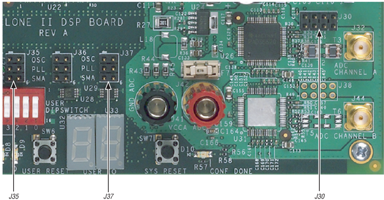
Figure 2–8. Locations of Jumpers J30, J35 & J37
