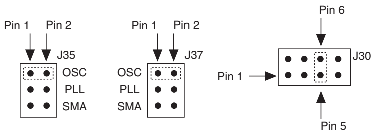
Figure 2–9. Jumper Connections for J35, J37 & J30
