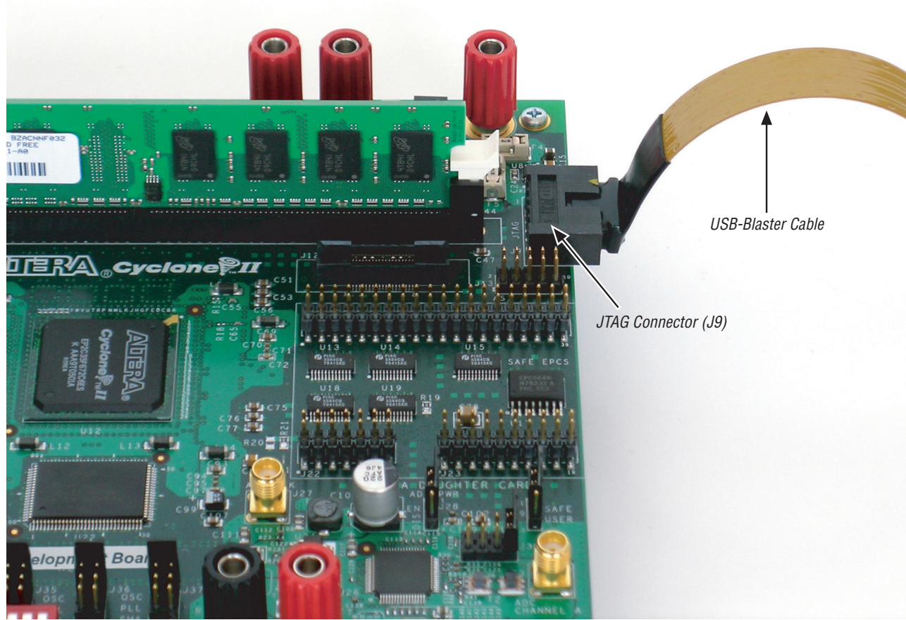
Figure 2–3. Connecting the USB-Blaster Download Cable to J9
