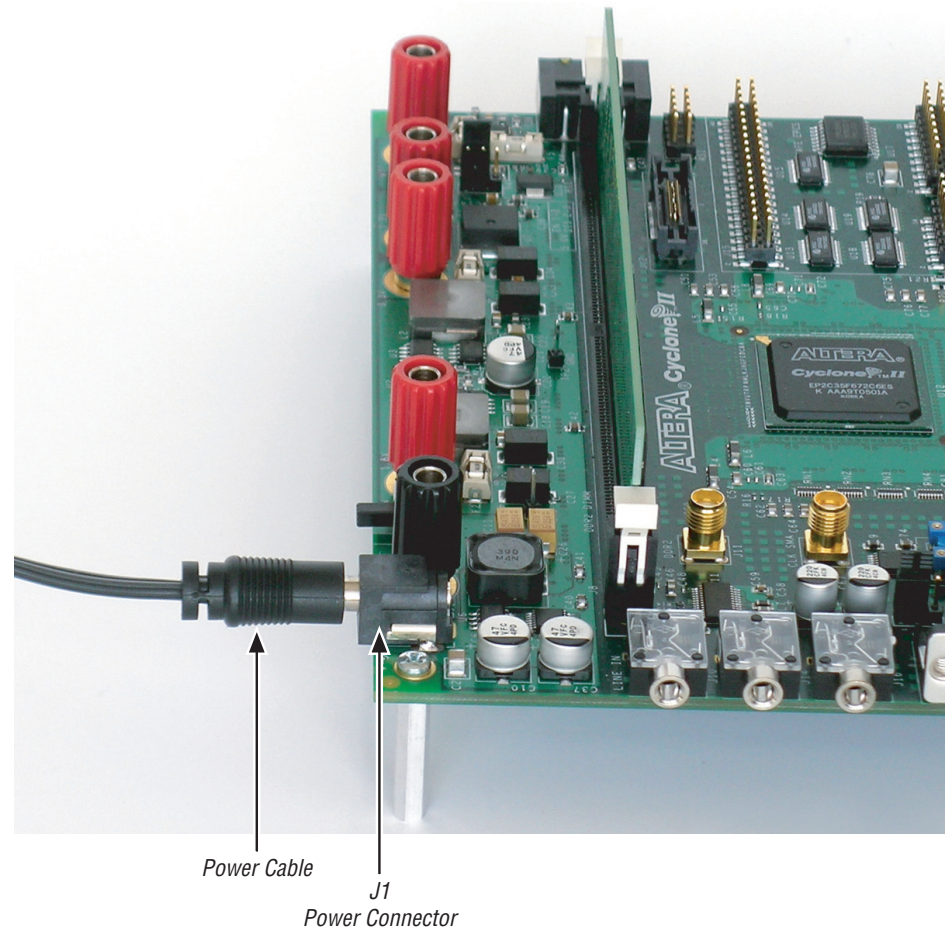
Figure 2-5. Connected Power Supply Cable
