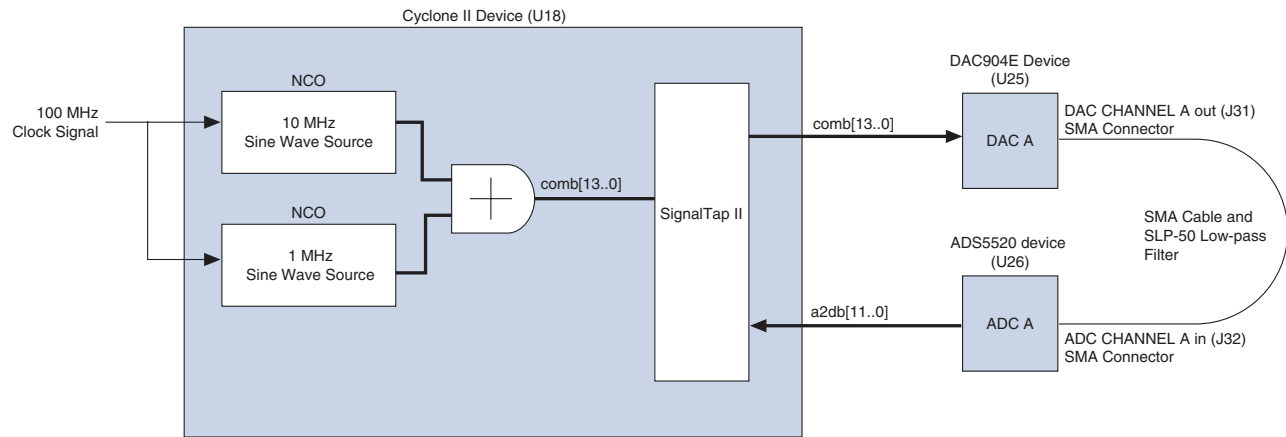
Figure 2–7. Factory Design Functional Block Diagram
