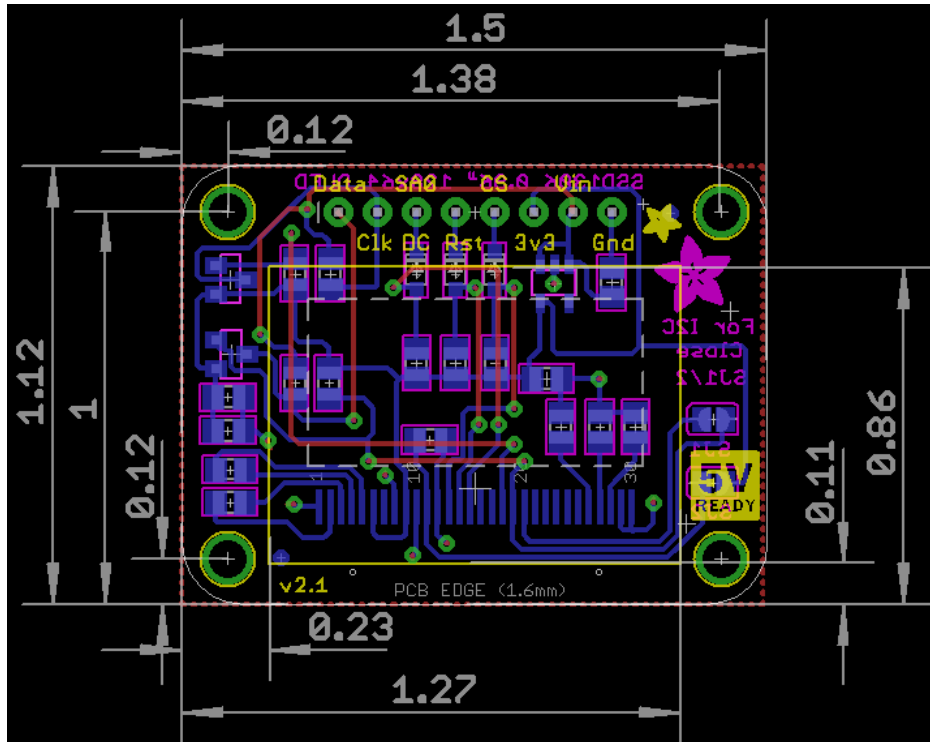
Schematic & Fabrication Print for 1.3" OLED
