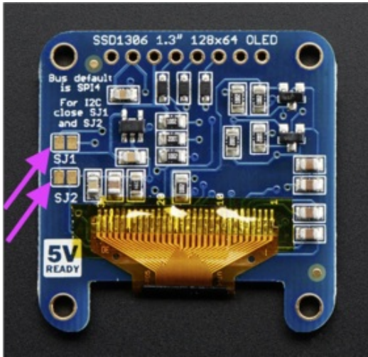
Adafruit 0.96" or 1.3" 128x64 OLED Display - SPI Wiring
