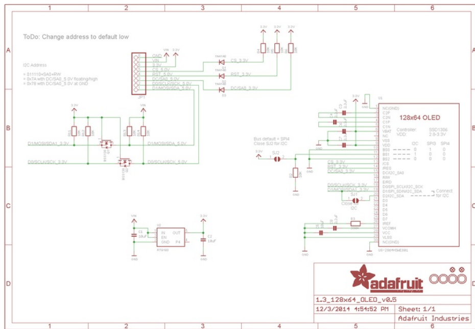
Schematic & Fabrication Print for 1.3" OLED
