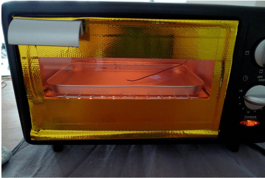
RocketNumberNine's reflow toaster project ( https://adafru.it/aLn )
