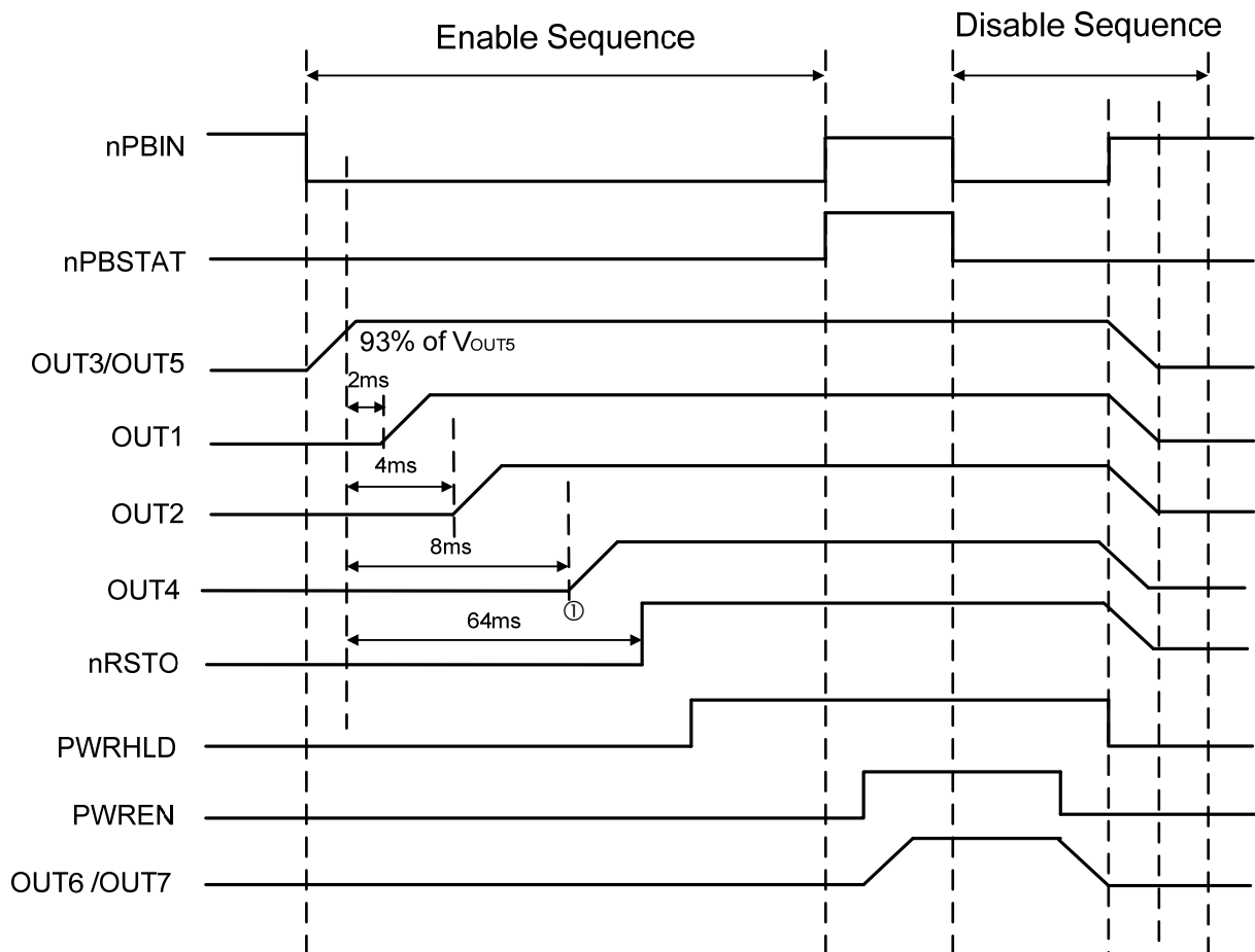
Figure 3: ACT8865QI305-T Enable/Disable Sequence
